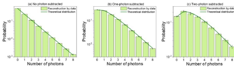
Fig. 1: Reconstructed photon-number distribution (green bars) and theoretical thermal distribution (green curve) in the case of no photon subtraction (a), one photon subtraction (b) and two photon subtraction (c).
